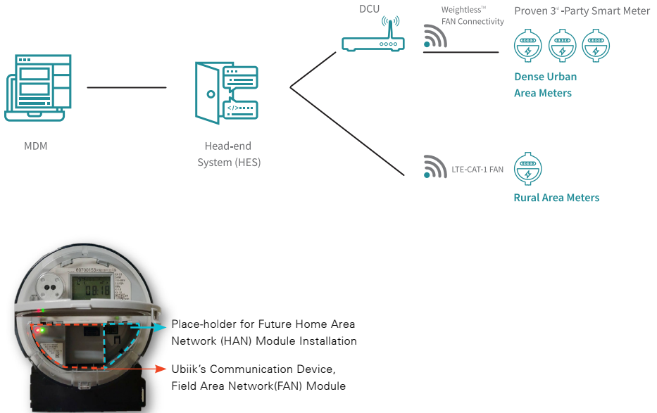
Figure 3: An example of how Ubiik's FAN solution fits into existing smart meters. On the top is a demonstration of Ubiik's LTE-Cat-1 and Weightless™ FAN connectivity architecture. On the bottom, the FAN installed in a meter. In Taiwan, future additional devices for higher frequency applications (e.g. HAN) can be added to smart meters.
