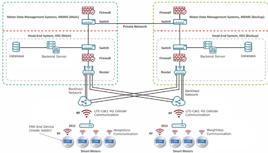
Figure 1: A general architecture of Ubiik's AMI infrastructure. Diagram sourced and modified from TPC [1]. This infrastructure consists of 5 main components starting from the FAN device (inside a smart meter) going up towards DCUs, a backhaul network, HES backend system, MDMS (and Frontend GUI). Note that in some cases, where device density is low, Ubiik FAN devices may communicate directly via cellular network.
